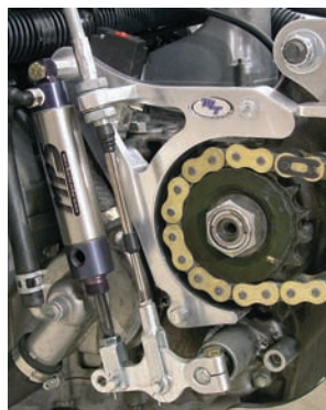
MANUAL LEVER SHIFTER CONTROL ASM (INCLUDES CABLE)
